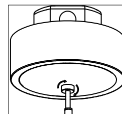
Figure 3: Canopy Mounting
