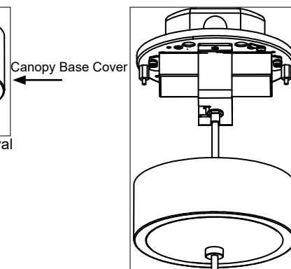
Figure 2: Base Mounting
