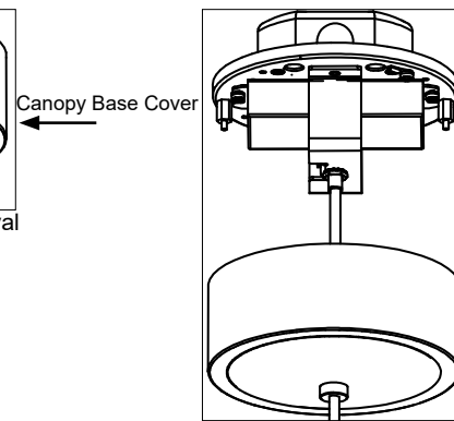
Figure 2: Base Mounting
