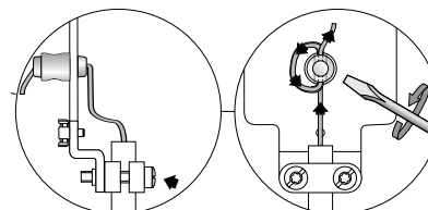
Figure 4: Cable Shortening
