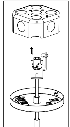
Figure 2: Base Mounting [1/2]
