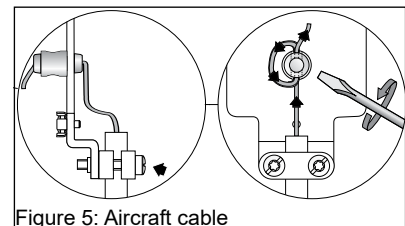
Figure 5: Aircraft cable
