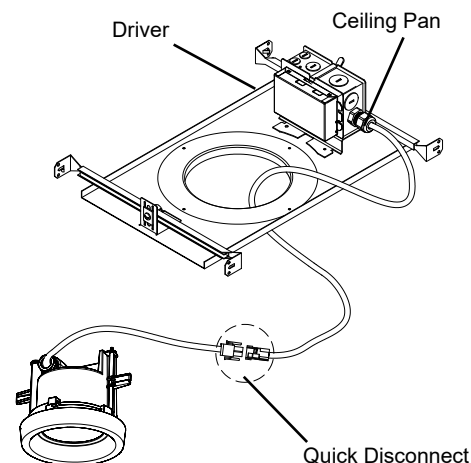
Figure 1: Ceiling pan for LED fixtures. Images are generic.
