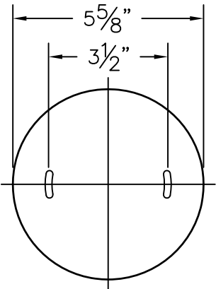
CANOPY MOUNTING PLATE
