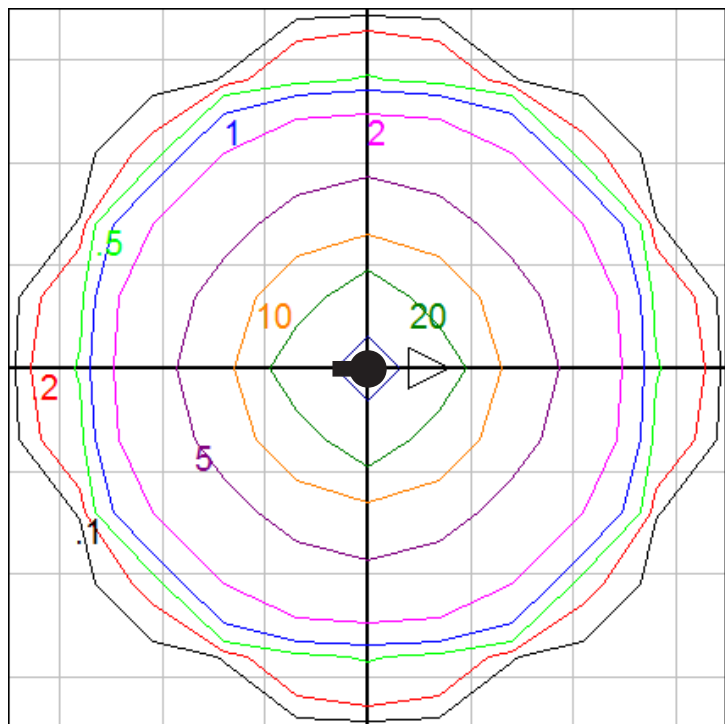
Wall Mount - Isofootcandle grid on floor Mounting Height = 10 ft. Grid Spacing = 2.5 ft.
