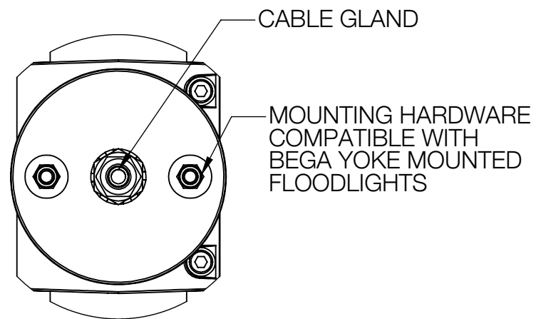
DETAIL A
