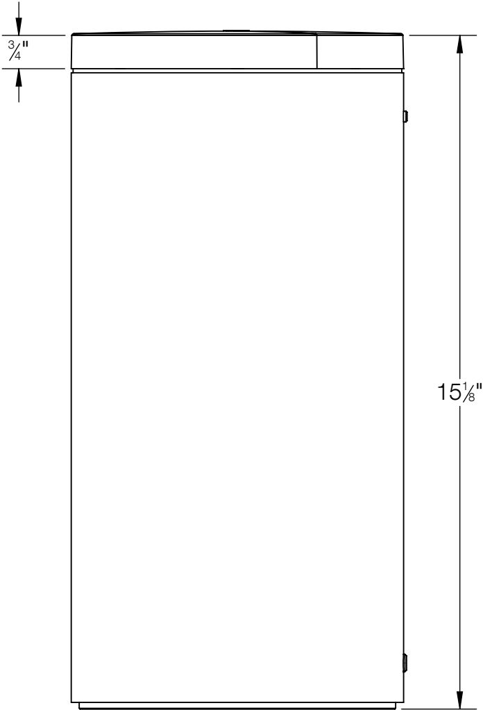
71127 SYSTEM BOLLARD HEAD SHOWN ON SYSTEM BOLLARD TUBE 99615 (NOT TO SCALE, TUBE SOLD SEPERATELY)
