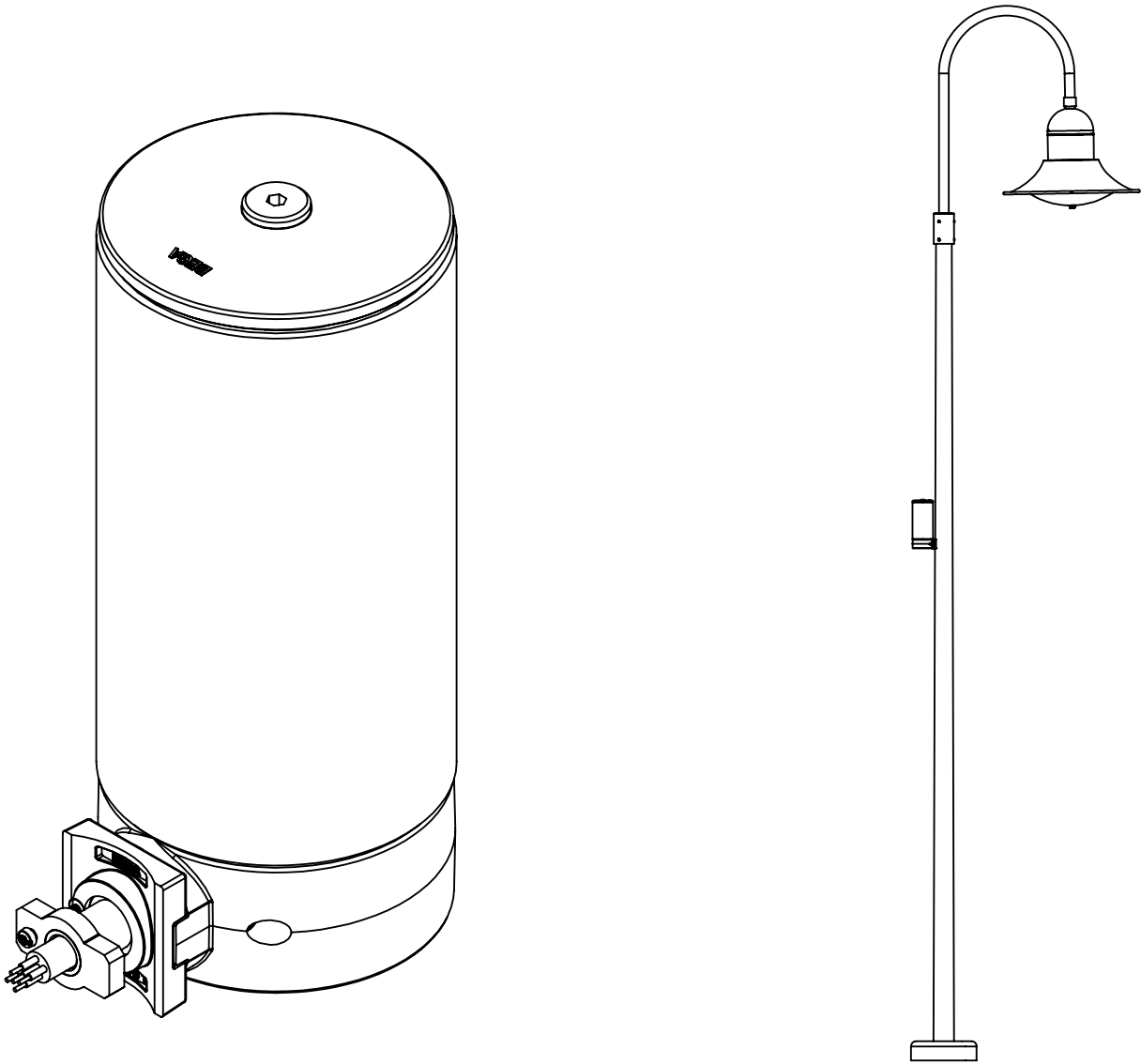
SHOWN INSTALLED ON BEGA POLE B14RHTS1 WITH POLETOP 77911 (SOLD SEPERATELY)
