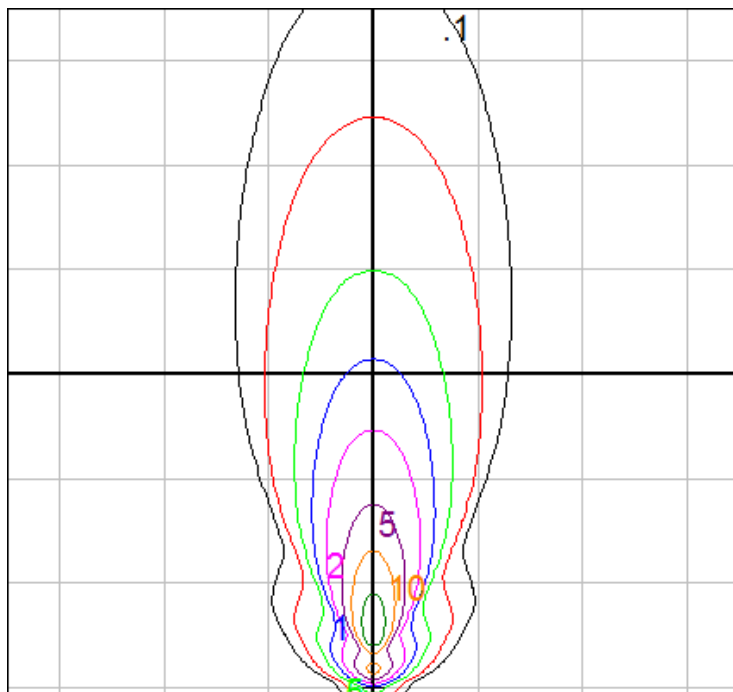
In-Grade Fixture - Isofootcandle Grid on Wall Fixture Setback = 1 ft. Grid Spacing = 5 ft.
