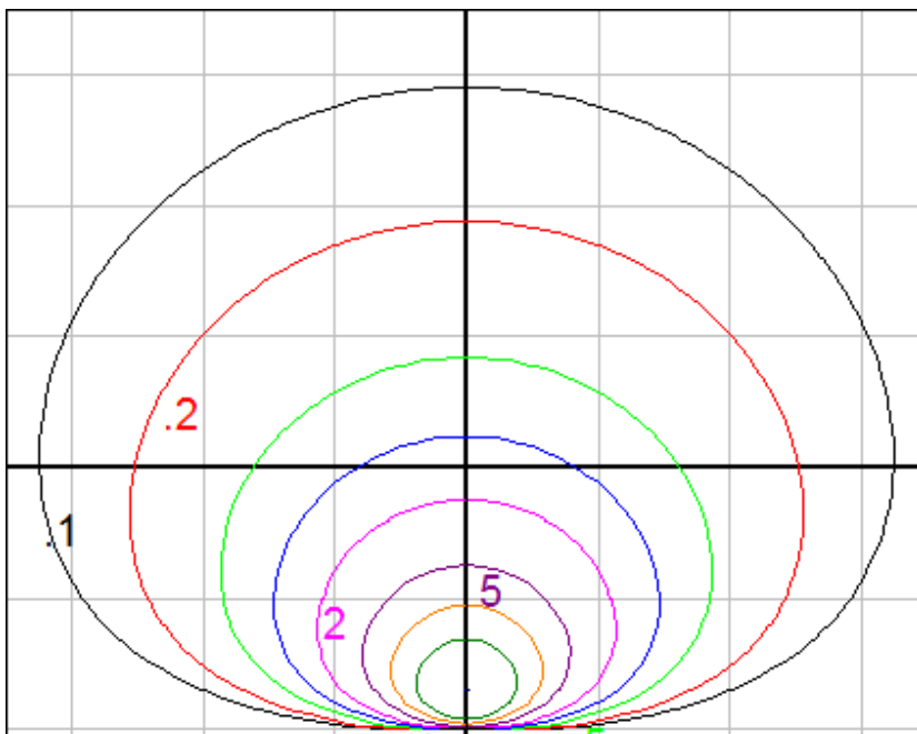
In-Ground Luminaire - Isofootcandle Diagram on Wall Fixture Setback = 1 ft. Grid Spacing = 2.5 ft.
