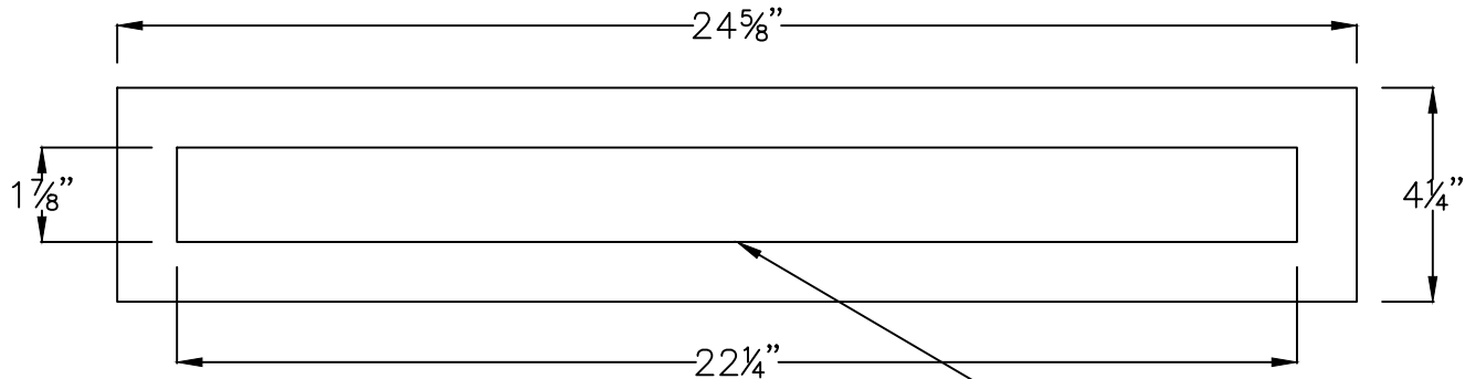
BACK BOX DETAIL
