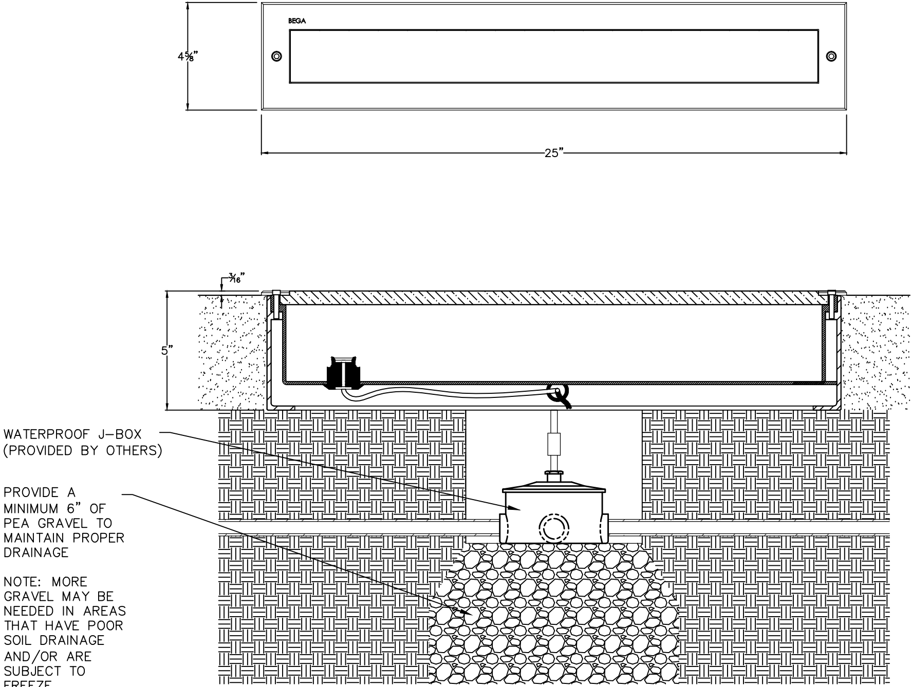
BACK BOX DETAIL
