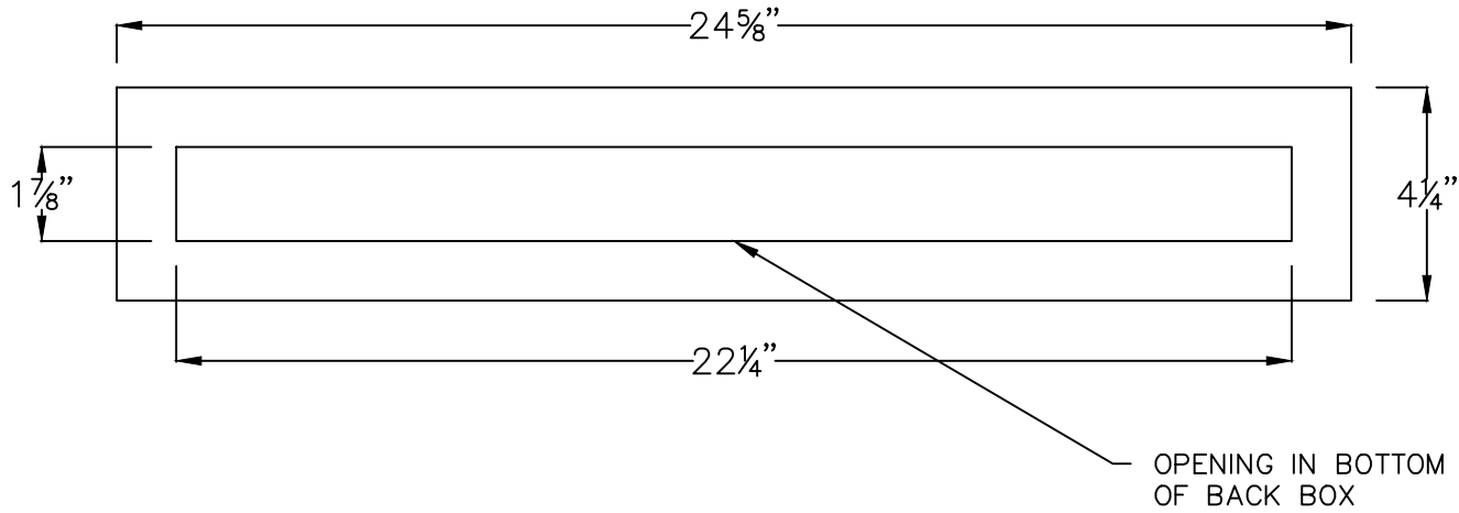
BACK BOX DETAIL
