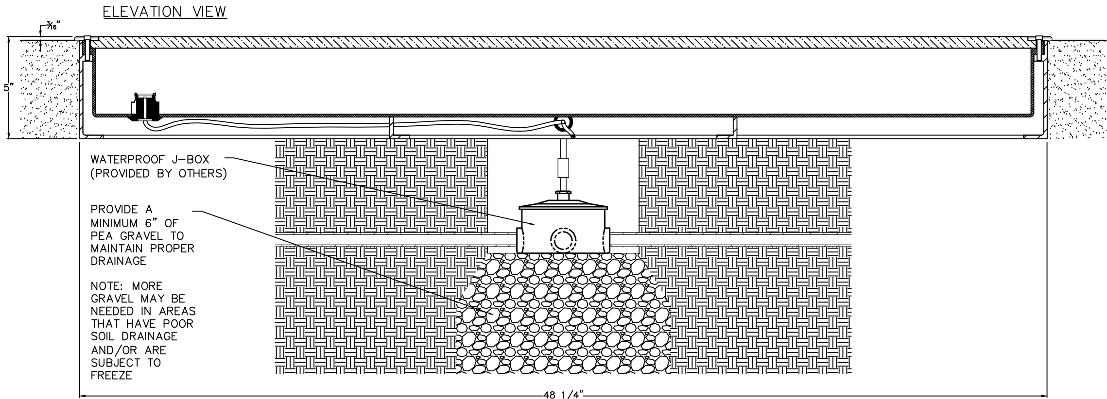
BACK BOX DETAIL
