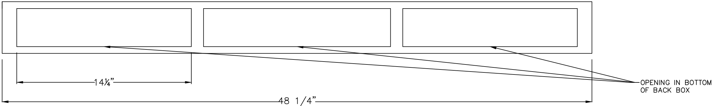
BACK BOX DETAIL
