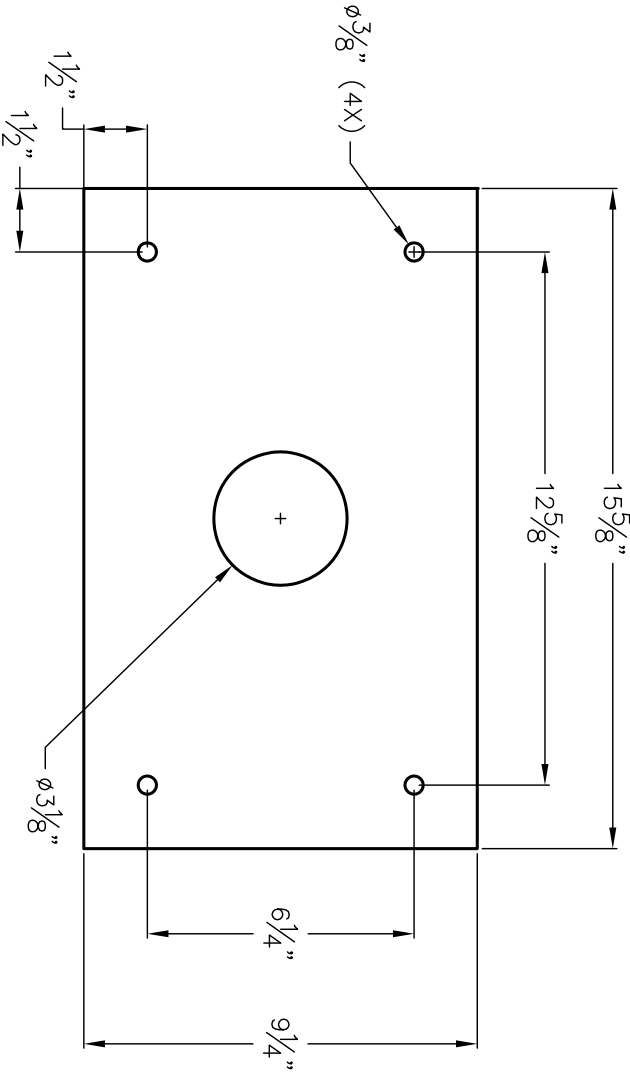
BASE MOUNTING DETAIL 79 808
