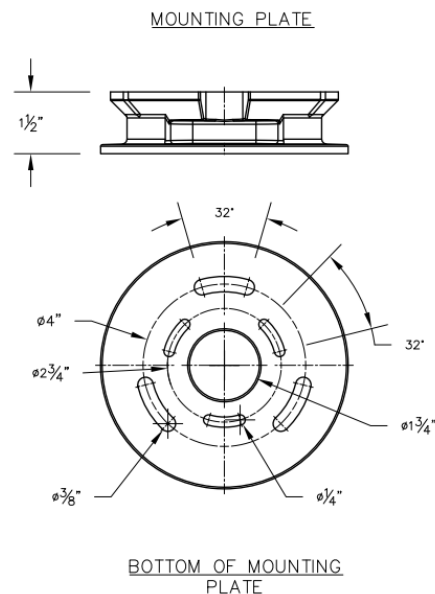
Figure 1: Anchorage Template
