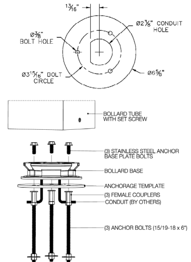
Figure 2: 70895 direct burial anchor installation:
