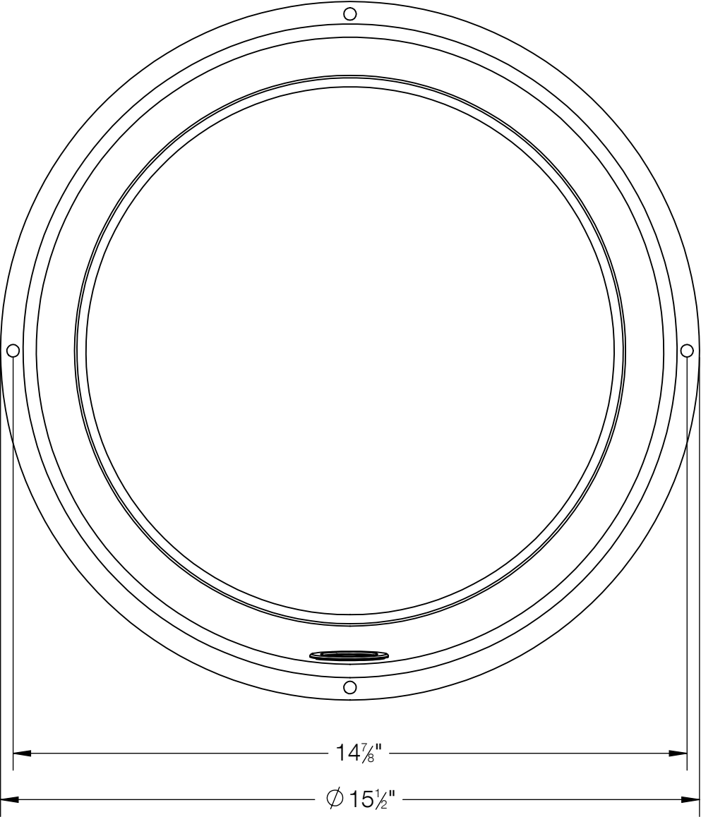
TOP VIEW
