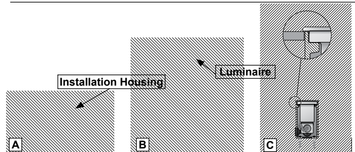
Figure 3: Installation
