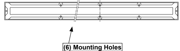
Figure 1: Mounting Holes
