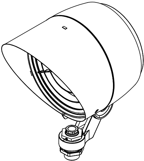
84215 SHOWN WITH 180° GLARE SHIELD ACCESSORY 71118 GLARE SHIELD IS ROTATABLE 360°
