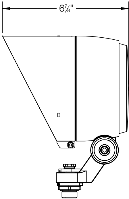
84215 SHOWN WITH 180° GLARE SHIELD ACCESSORY 71118 GLARE SHIELD IS ROTATABLE 360°
