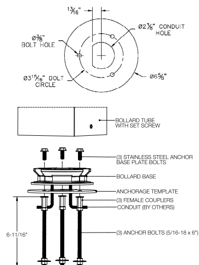
Figure 2: 70895 direct burial anchor installation:
