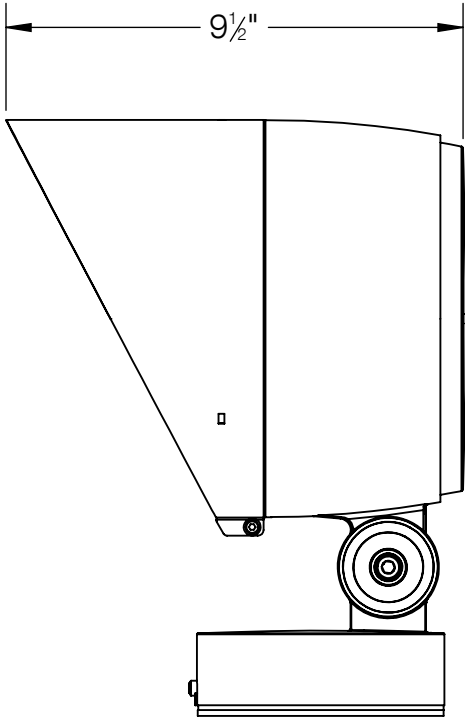
84222 SHOWN WITH 180° GLARE SHIELD ACCESSORY 71121 GLARE SHIELD IS ROTATABLE 360°
