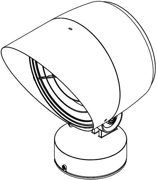
84222 SHOWN WITH 180° GLARE SHIELD ACCESSORY 71121 GLARE SHIELD IS ROTATABLE 360°
