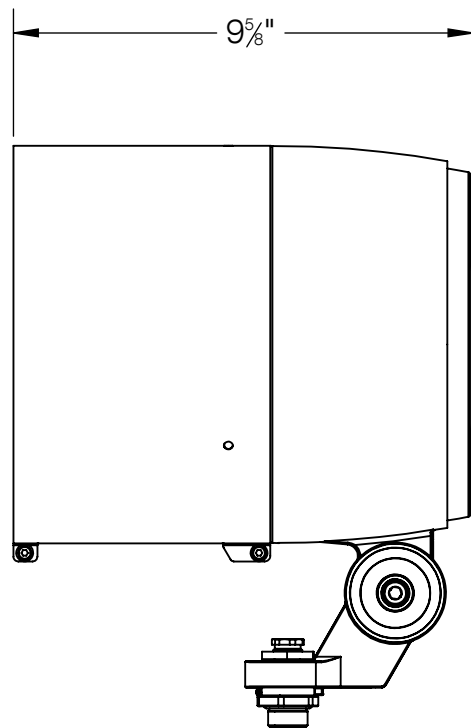
84227 SHOWN WITH 360° GLARE SHIELD ACCESSORY 79831 GLARE SHIELD IS ROTATABLE 360°
