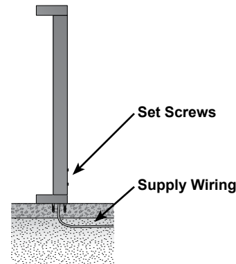
Figure 3: Base Details
