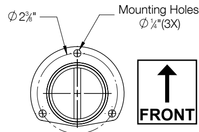
Anchorage Detail
