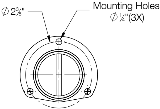
Anchorage Detail
