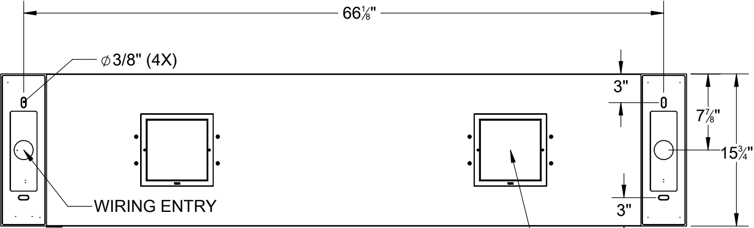
BOTTOM VIEW
