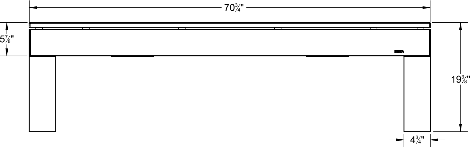
FRONT VIEW
