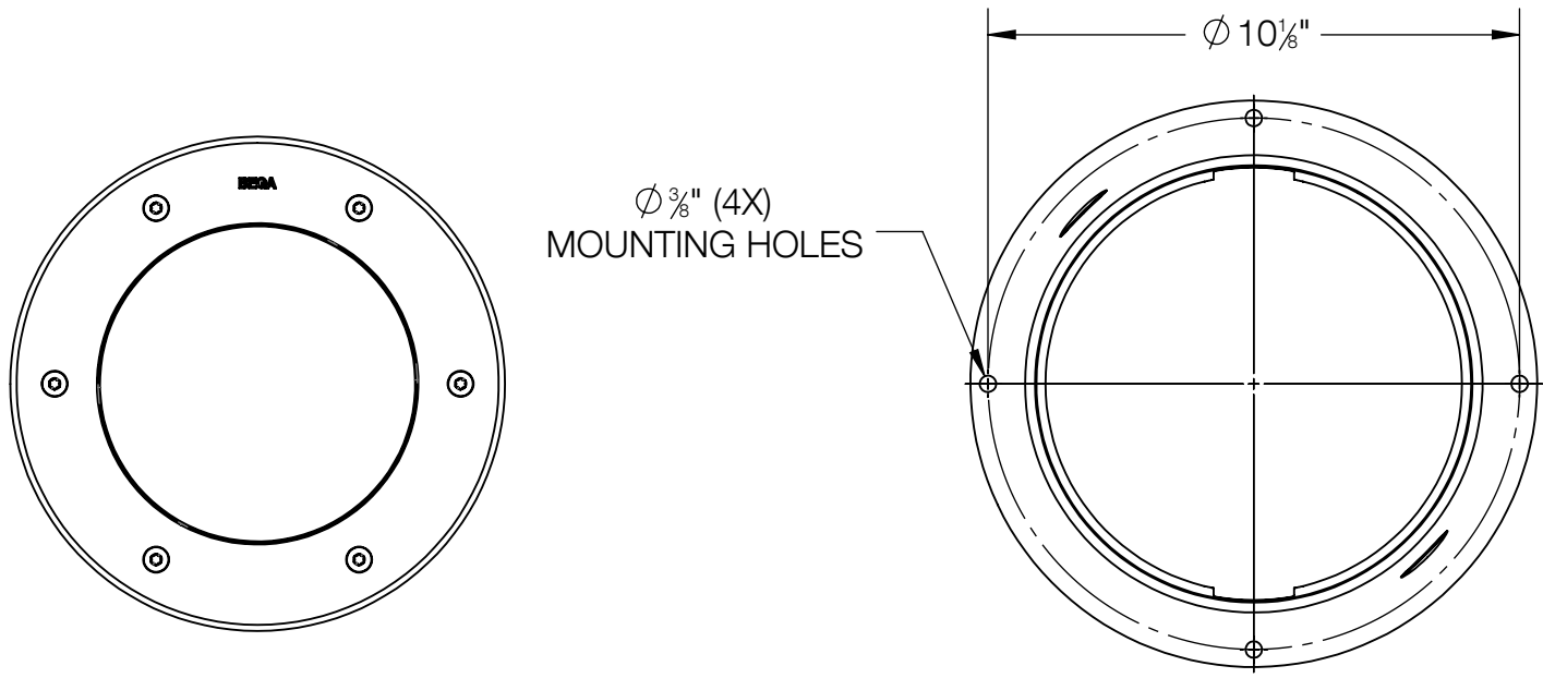
OUTER HOUSING DETAIL
