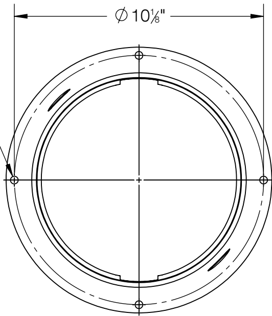
OUTER HOUSING DETAIL
