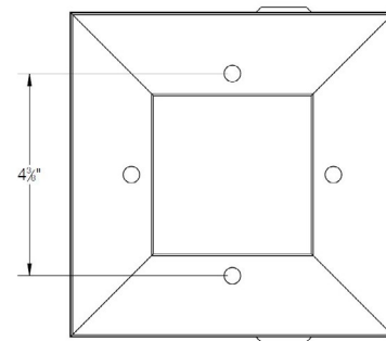
Figure 2: Mounting hole locations
