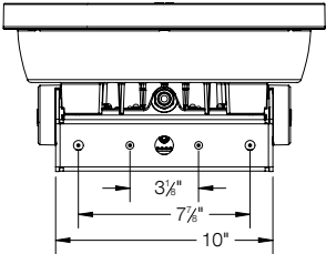
Figure 1: Yolk Mounting Detail
