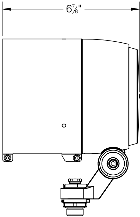
84330 SHOWN WITH 360° GLARE SHIELD ACCESSORY 79829 GLARE SHIELD IS ROTATABLE 360°
