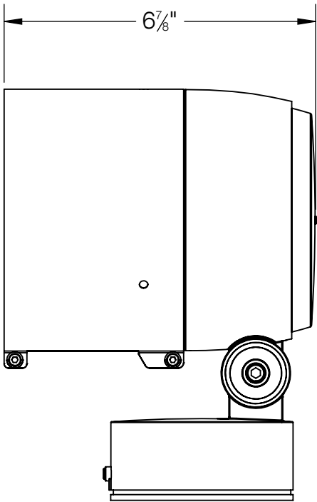
84332 SHOWN WITH 360° GLARE SHIELD ACCESSORY 79829 GLARE SHIELD IS ROTATABLE 360°
