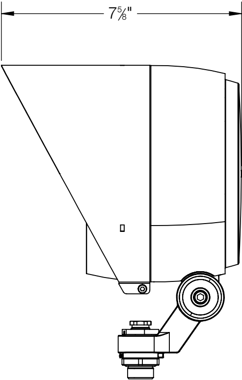
84358 SHOWN WITH 180° GLARE SHIELD ACCESSORY 71111 GLARE SHIELD IS ROTATABLE 360°
