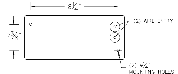
Figure 2: Mounting Detail
