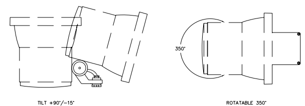
Figure 3: Floodlight Adjustability
