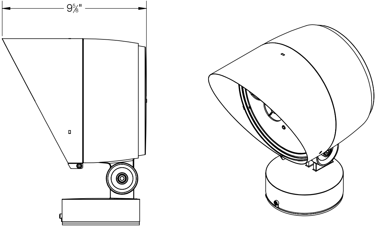
84409 SHOWN WITH 180° GLARE SHIELD ACCESSORY 71121 GLARE SHIELD IS ROTATABLE 360°
