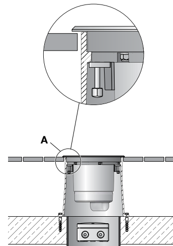
Figure 2: Faceplate Detail
