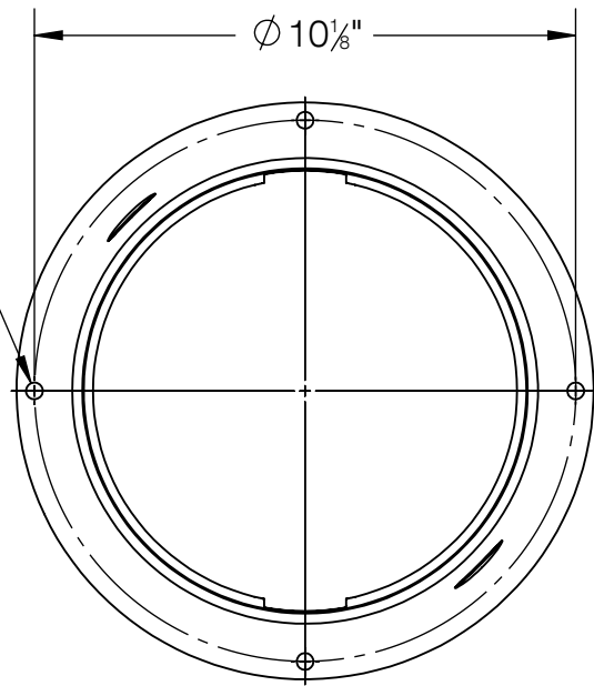
OUTER HOUSING DETAIL
