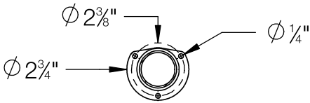
MOUNTING FOOT DETAIL
