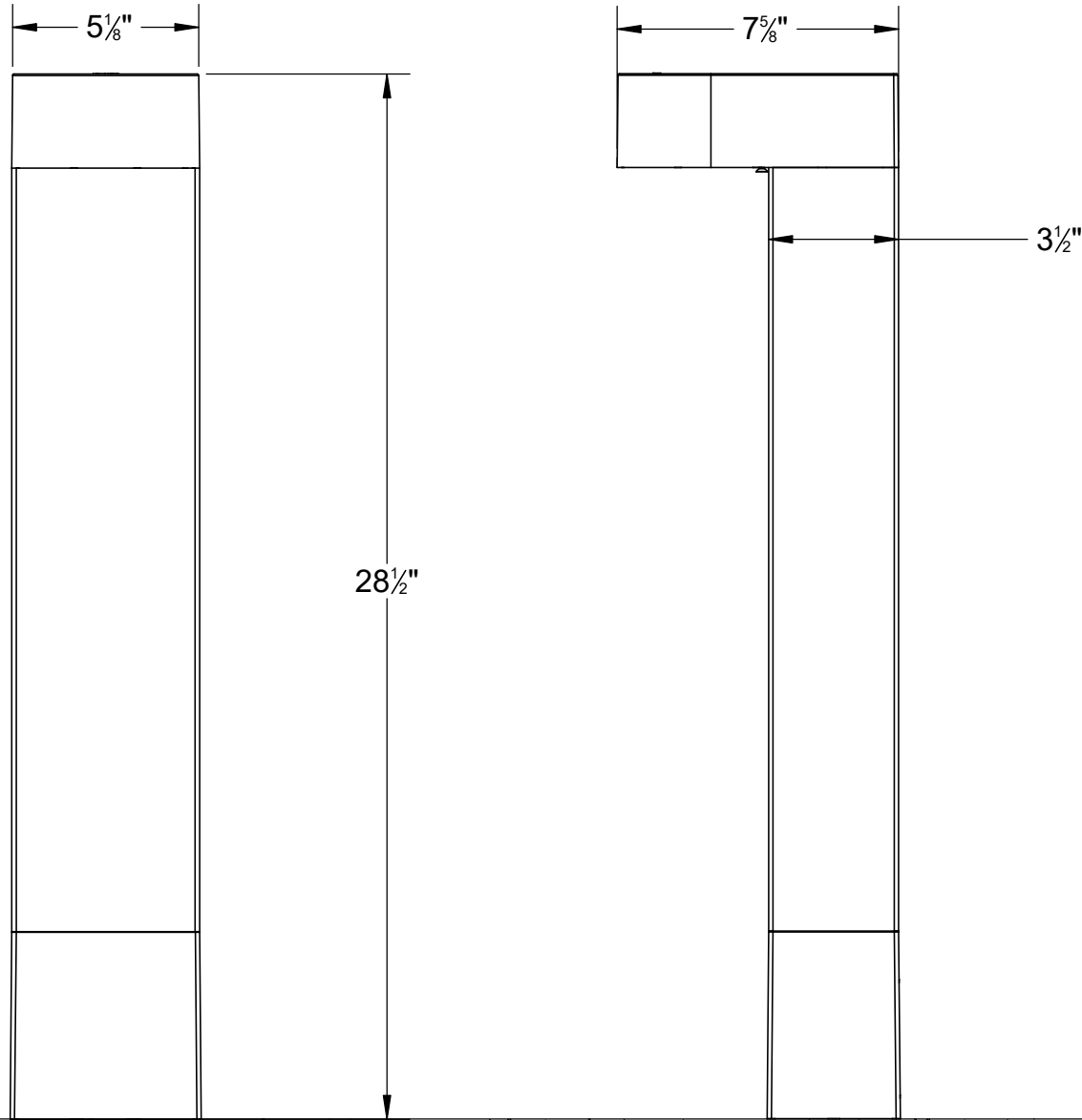
MOUNTING FOOT DETAIL
