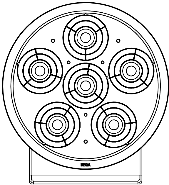
84524 SHOWN WITH 71109 - CONCENTRIC RING LOUVER
