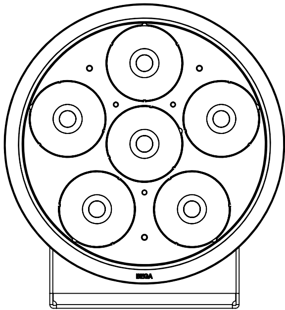
84524 SHOWN WITH 79510 - 360° GLARE SHIELD
