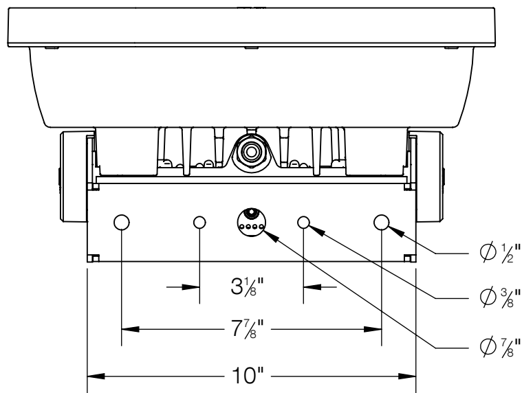
MOUNTING DETAIL
