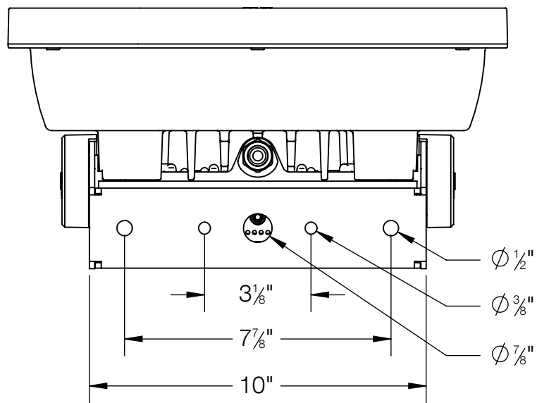
MOUNTING DETAIL
