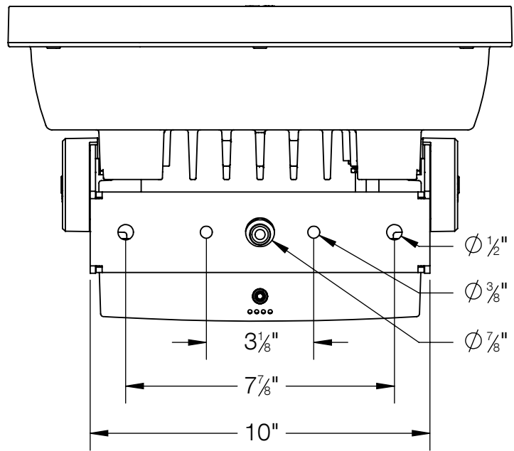
MOUNTING DETAIL
