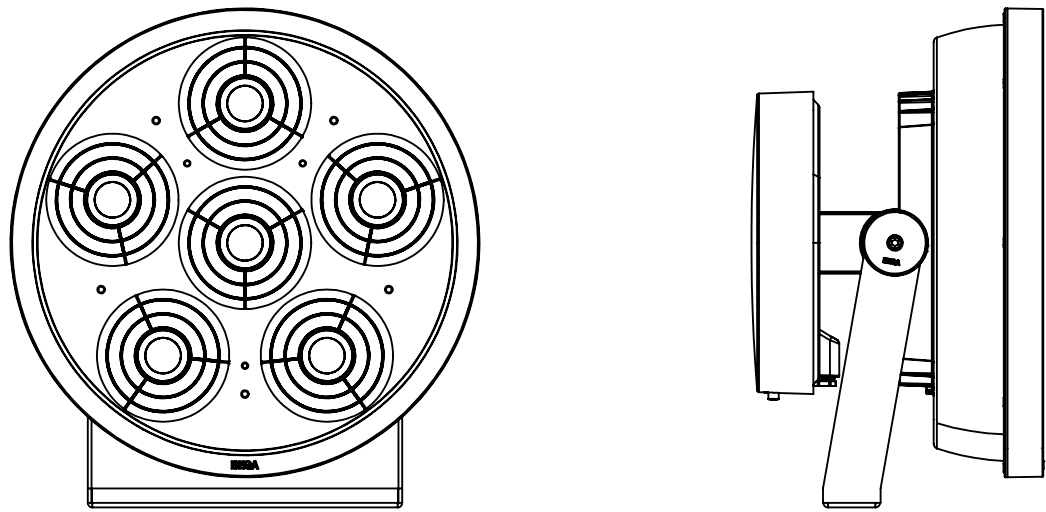
84551 SHOWN WITH 71105 - CONCENTRIC RING LOUVER
