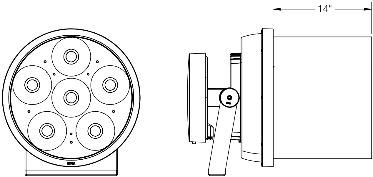
84551 SHOWN WITH 79509 - 360° GLARE SHIELD
