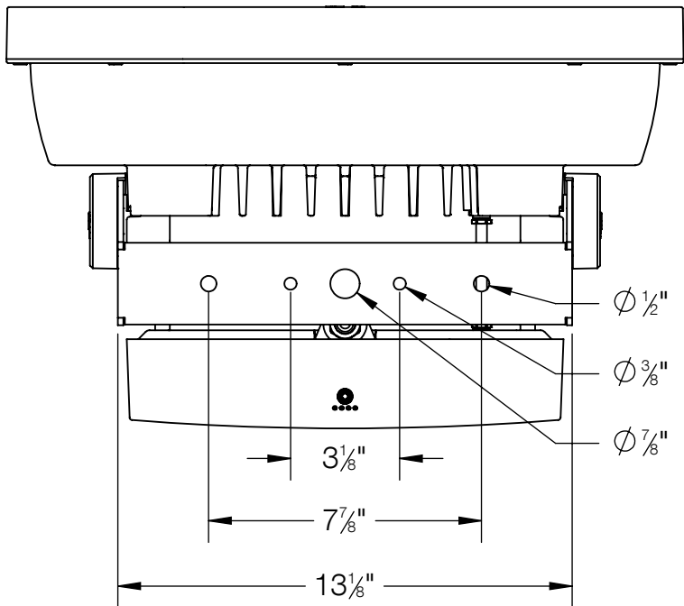
MOUNTING DETAIL
