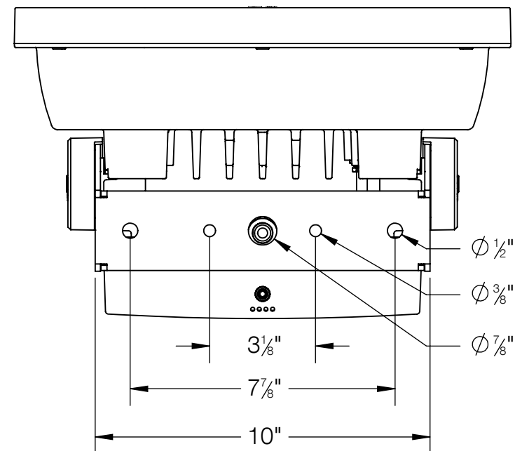
MOUNTING DETAIL
