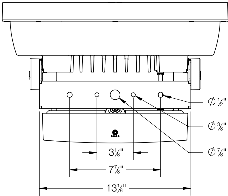
MOUNTING DETAIL
