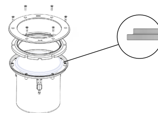
Figure 4: Faceplate Removal (Generic Image)
