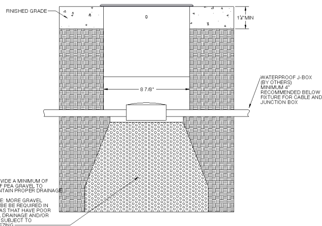
Figures 2 & 3: Installation Clamping system
