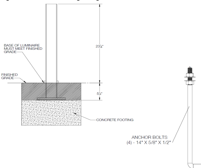
Figure 2: 79 828 Anchorage Diagram
