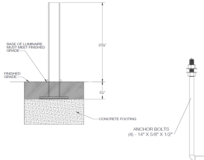
Figure 2: 79 828 Anchorage Diagram
