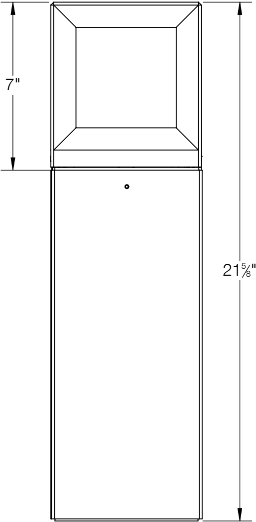
84680 SYSTEM BOLLARD HEAD SHOWN ON SYSTEM BOLLARD TUBE 84002 (NOT TO SCALE, TUBE SOLD SEPERATELY)
