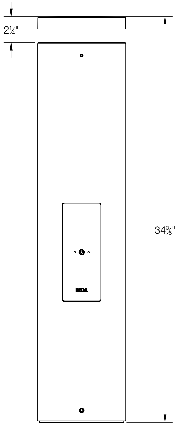
84704 SYSTEM BOLLARD HEAD SHOWN ON SYSTEM BOLLARD TUBE 99622 (NOT TO SCALE, TUBE SOLD SEPERATELY)
